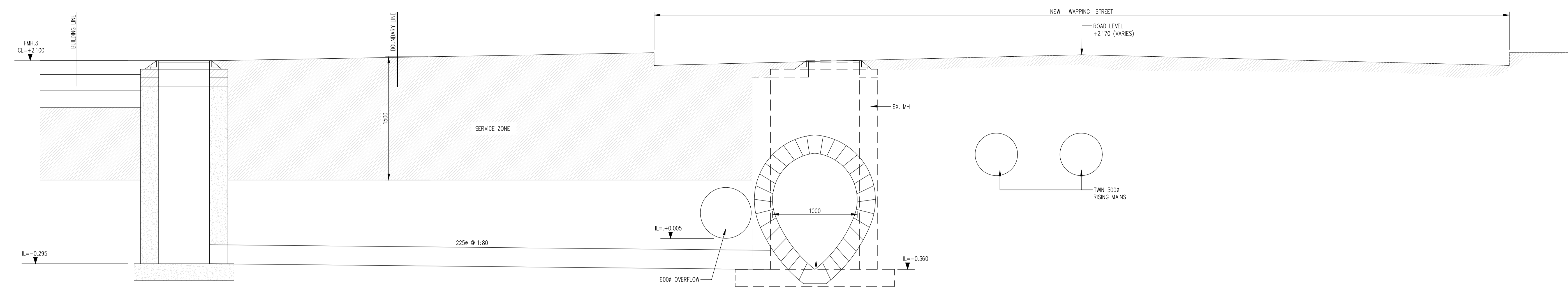
SECTION X-X (INDICATIVE ONLY) SCALE 1/25
